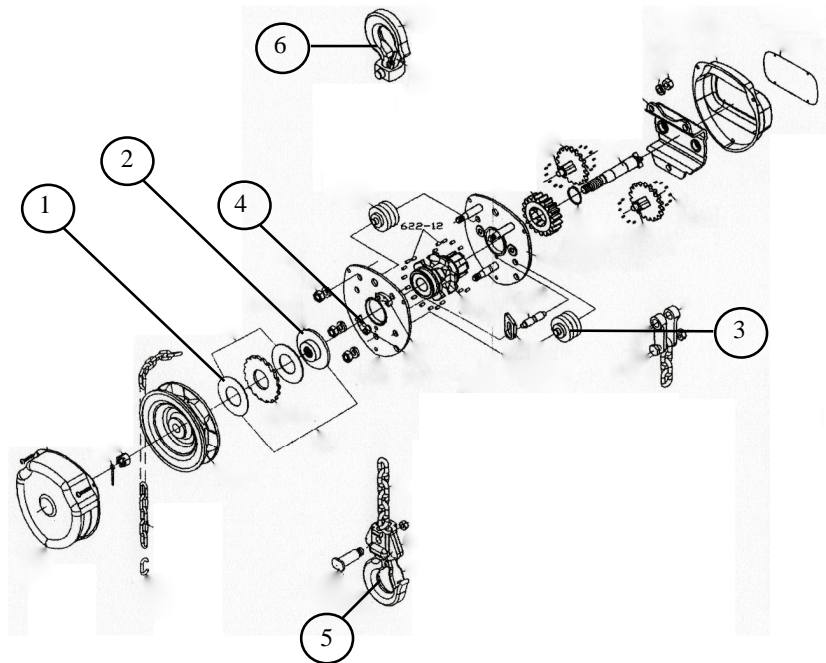
Principle sketch
